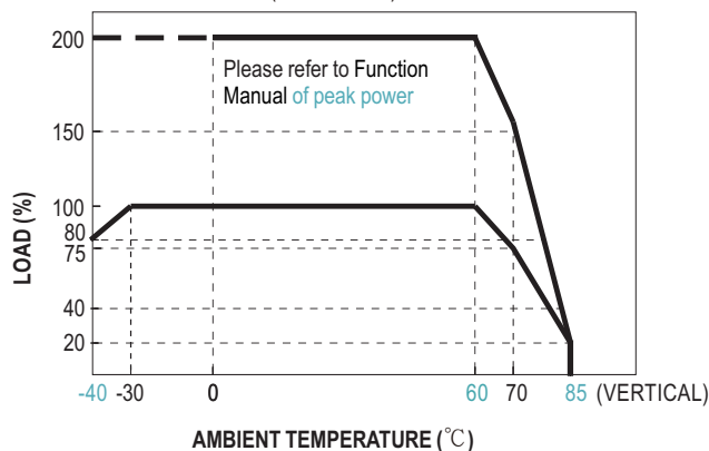
Suitable for 220/230/240/277Vac System (180~305Vac)
